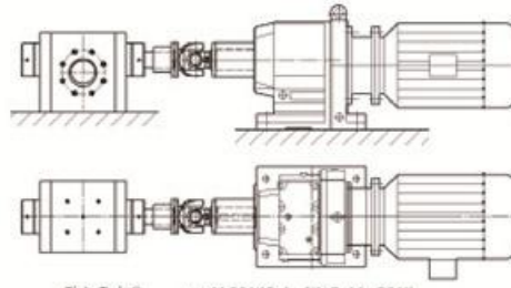
A型水平安装 A HORIZONTAL INSTALLATION
